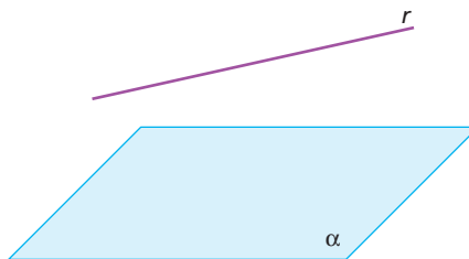
r \cap \alpha = \emptyset
