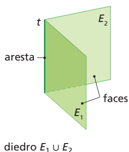
diedro E_1 \cup E_2
