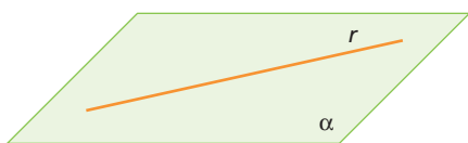
r \subset \alpha
