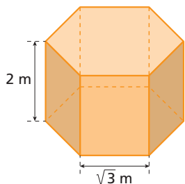
prisma hexagonal regular
