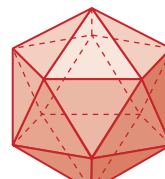
icosaedro regular
