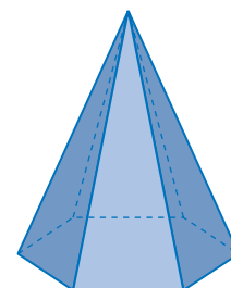
pirâmide hexagonal
