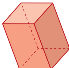
prisma quadrangular
