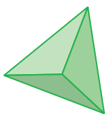
tetraedro regular
