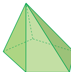
pirâmide pentagonal
