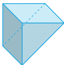
prisma triangular
